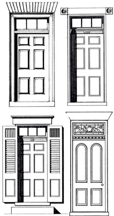
Figure 21: Typical rowhouse door styles.
