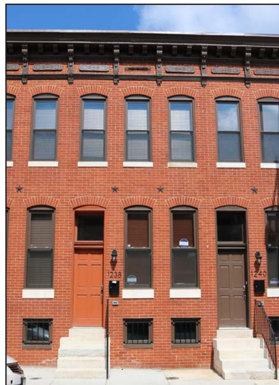
Figure 5: RECOMMENDED - Repointed brick that replicates the color, texture, composition, and tooling of the historic mortar.
