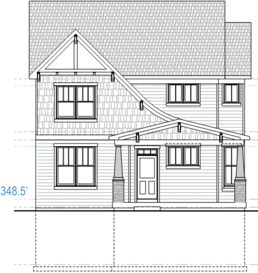
Street Elevation 348.5'
